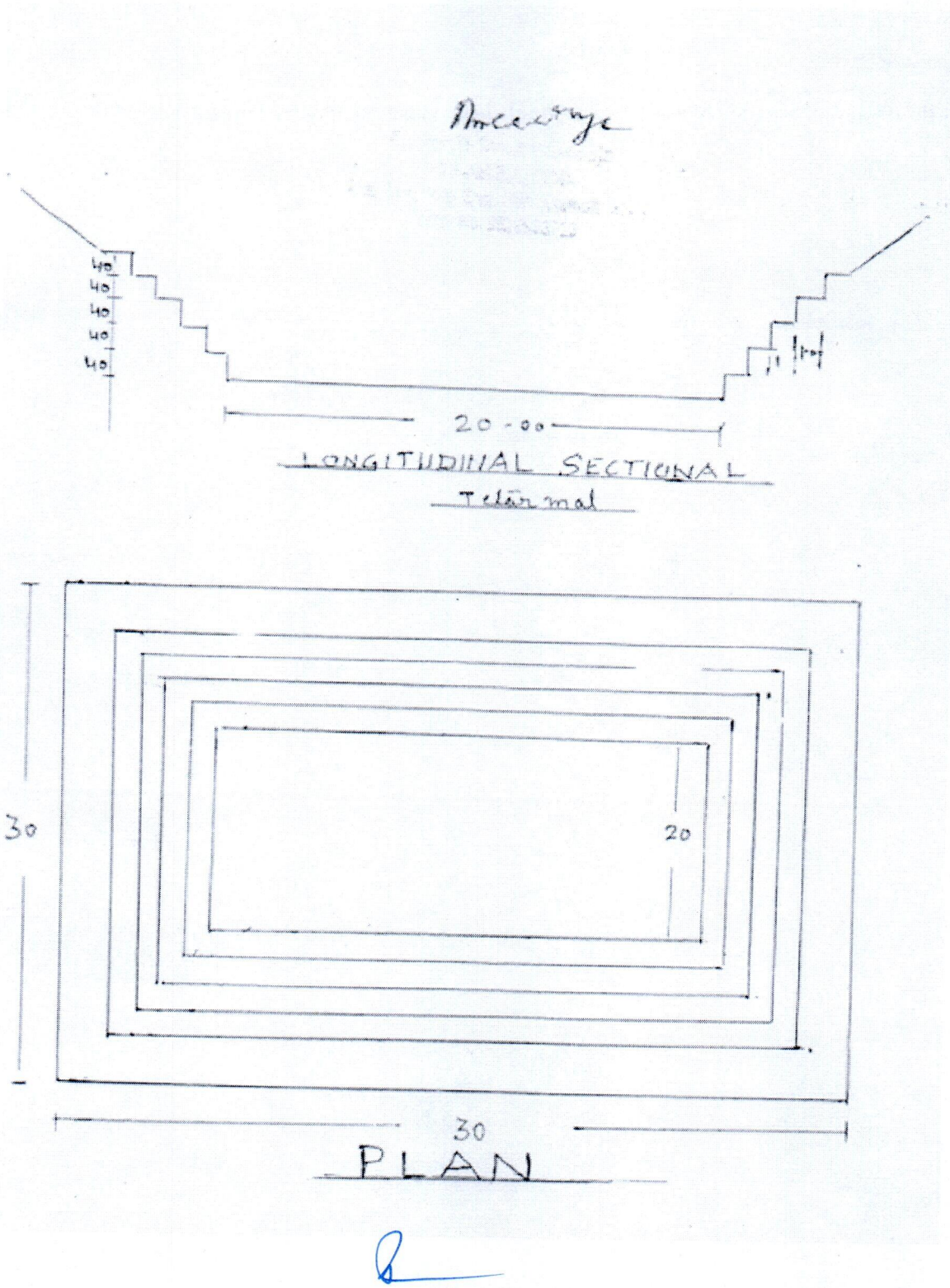
Figure for (C1). Construction of waste weir of Banbaheda village of Bhoura Forest Range (MP)
