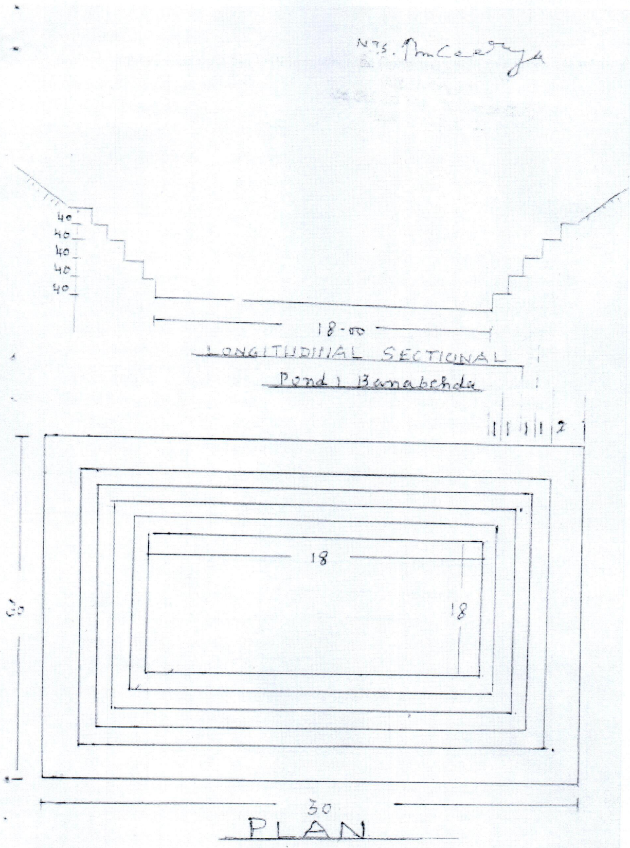
Figure for (A). Deepening of pond at Banbaheda village of Bhoura Forest Range (MP)
